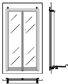
LR10 OVERALL SIZE = 820 x 1430
