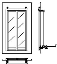
LR11 OVERALL SIZE = 593 x 1021
