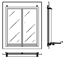
LR5 OVERALL SIZE = 972 x 1169
