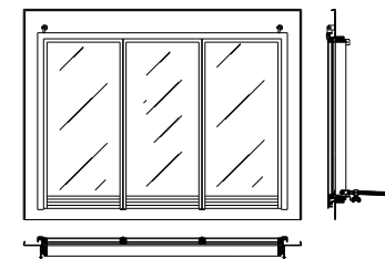
LR12 OVERALL SIZE = 1481 x 1124
