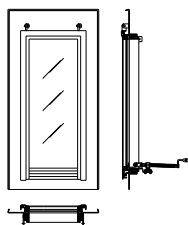
LR9 OVERALL SIZE = 537 x 1065
