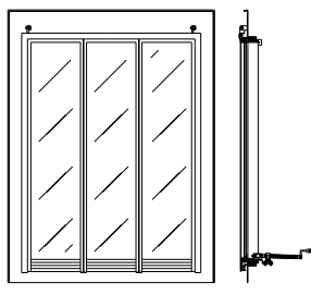
LR6 OVERALL SIZE = 1124 x 1481
